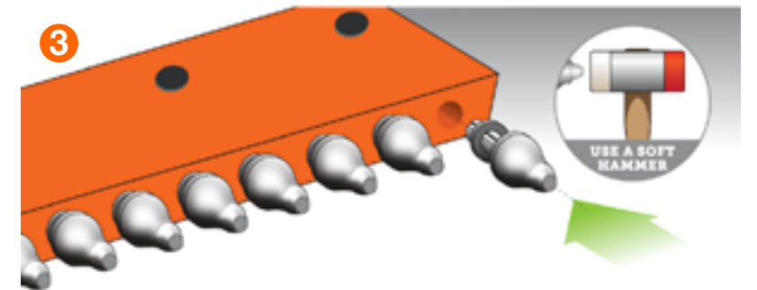
USE A SOFT HAMMER TO SET THE BITS INTO THE MOUNTING HOLES - A HARD SURFACE HAMMER COULD DAMAGE THE BIT'S HARDFACING
