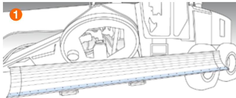
RAISE THE SADDLE TO MAKE THE CUTTING EDGE EASILY ACCESSIBLE. CLEAN MOLDBOARD SURFACES THOROUGHLY.
